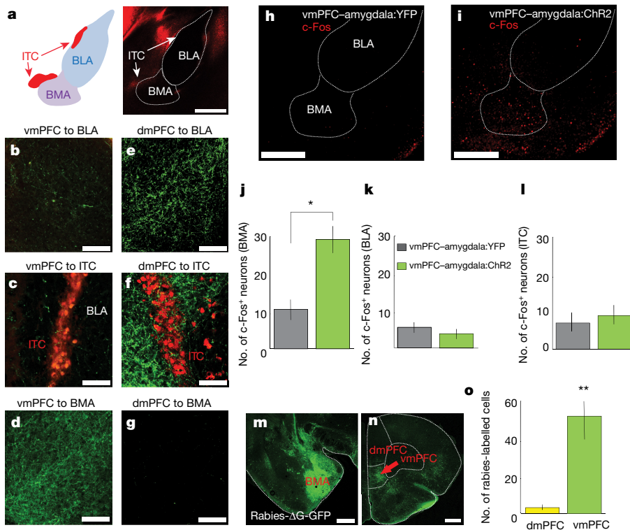
Figure 3 | Basomedial amygdala: major target of vmPFC in amygdala. a , Left: location of amygdala nuclei. Right: lox -tdTomato reporter line crossed with EY266 D1R:Cre line for ITC visualization. Scale bar, 500 \mu m. b–d , AAV5-CamK2 \alpha :ChR2-YFP injected in vmPFC; vmPFC fibres imaged in BLA ( b ), ITC ( c ) and BMA ( d ). a–d , Representative images from one mouse chosen out of n = 7 mice. e–g , Same as b–d , but for dmPFC. e–g , Representative images from one mouse chosen out of n = 7 mice. Scale bars, 50 \mu m ( c , f ); 100 \mu m ( b , e , d , g ). h–l , c-Fos-expressing cells (red) counted in BMA ( j ), BLA ( k ) and ITCs ( l ) following vmPFC-amygdala activation; increased c-Fos can be seen in BMA of vmPFC-amygdala:ChR2 mice. n = 5 mice, for each group, 4 slices per mouse. m–o , Rabies- \Delta G-GFP injected in BMA ( m ); retrogradely labelled cells counted ( n–o ). n = 4 mice ( o ). Scale bar, 500 \mu m ( h , i , m , n ). * P < 0.05 , ** P < 0.01 , two-sided Wilcoxon test. Error bars, mean \pm s.e.m.
