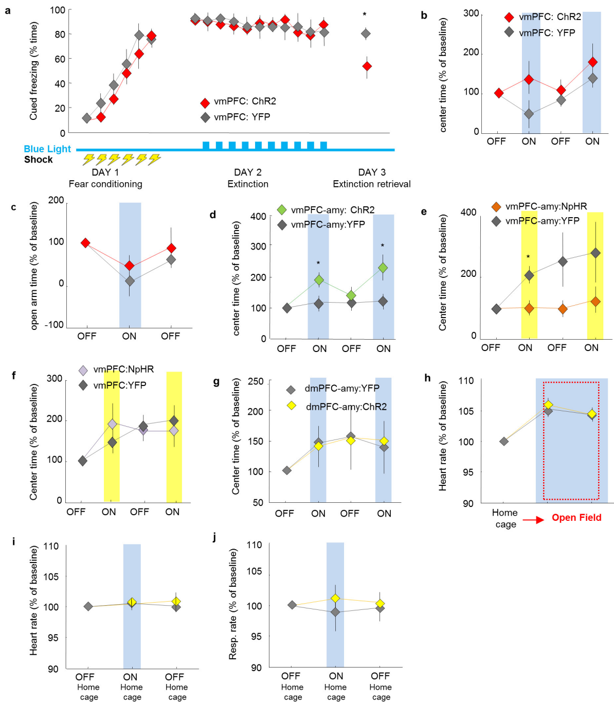
Extended Data Figure 2 | Optogenetic manipulations involving the mPFC and its projections in fear and anxiety paradigms. a , Mice were fear conditioned to six tone-shock (0.7 mA, 2-s shocks) pairings on day 1 (fear acquisition). On day 2 (fear extinction) animals were exposed to the tone in a different context for 11 trials. Blue light was delivered only on day 2, for trials 2–11. vmPFC:ChR2 mice froze less than control mice during day 3 (extinction retrieval). b , c , Blue light delivery did not change avoidance of open spaces in vmPFC:ChR2 mice relative to control mice in the open field ( b ) or the EPM ( c ). n = 7 vmPFC:ChR2 and 7 vmPFC:YFP mice ( a–c ). d , Excitation of the vmPFC–amygdala projection with blue light increased exploration of the centre of the open field in vmPFC–amygdala:ChR2 mice relative to controls. Two-way repeated measures ANOVA, opsin \times epoch interaction, F_{3,68} = 3.1 , P = 0.03 , post hoc Wilcoxon rank sum test P = 0.002 . n = 12 vmPFC–amygdala:ChR2 and 13 vmPFC–amygdala:YFP mice.
